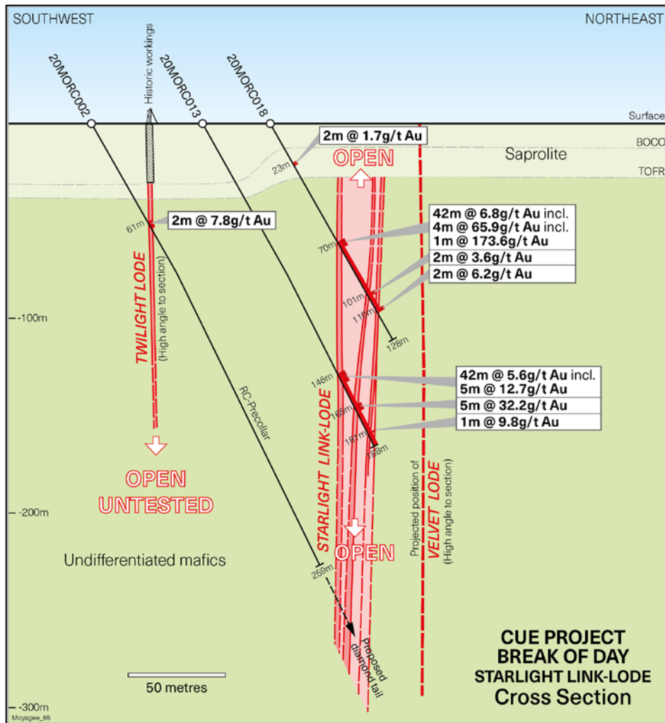
Figure 3: Cross-section of Starlight link-lobe at Break of Day
