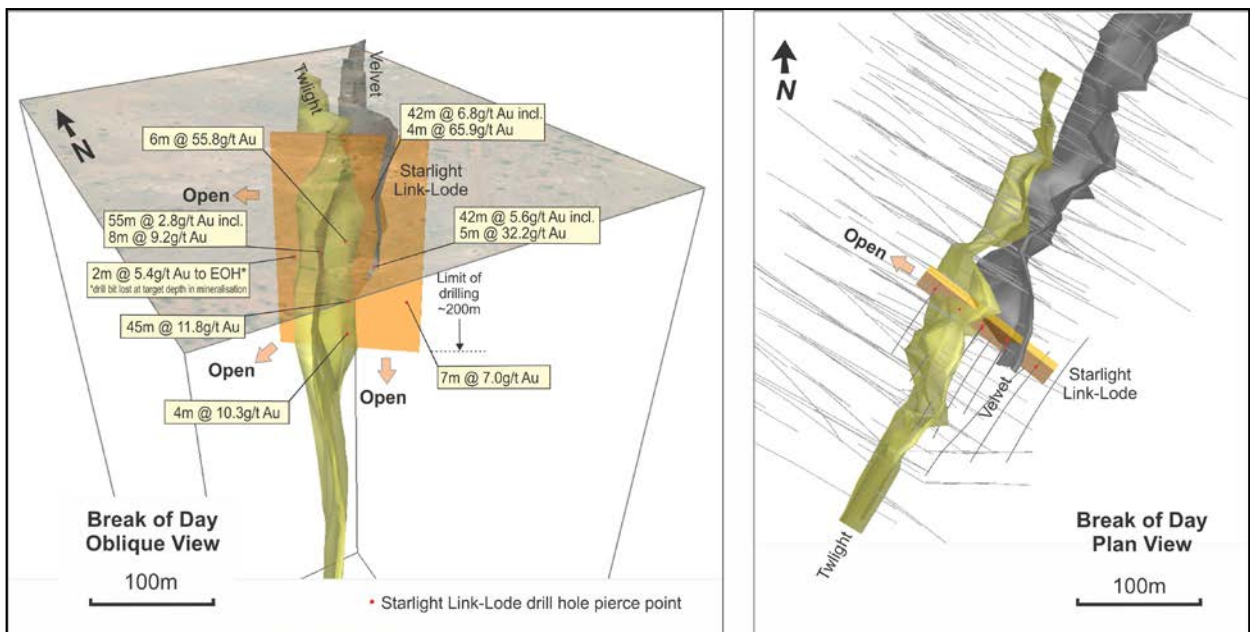
Figure 4: Schematic diagrams showing the location and orientation of the new Starlight link-lobe with respect to the Twilight and Velvet gold lodes at Break of Day
