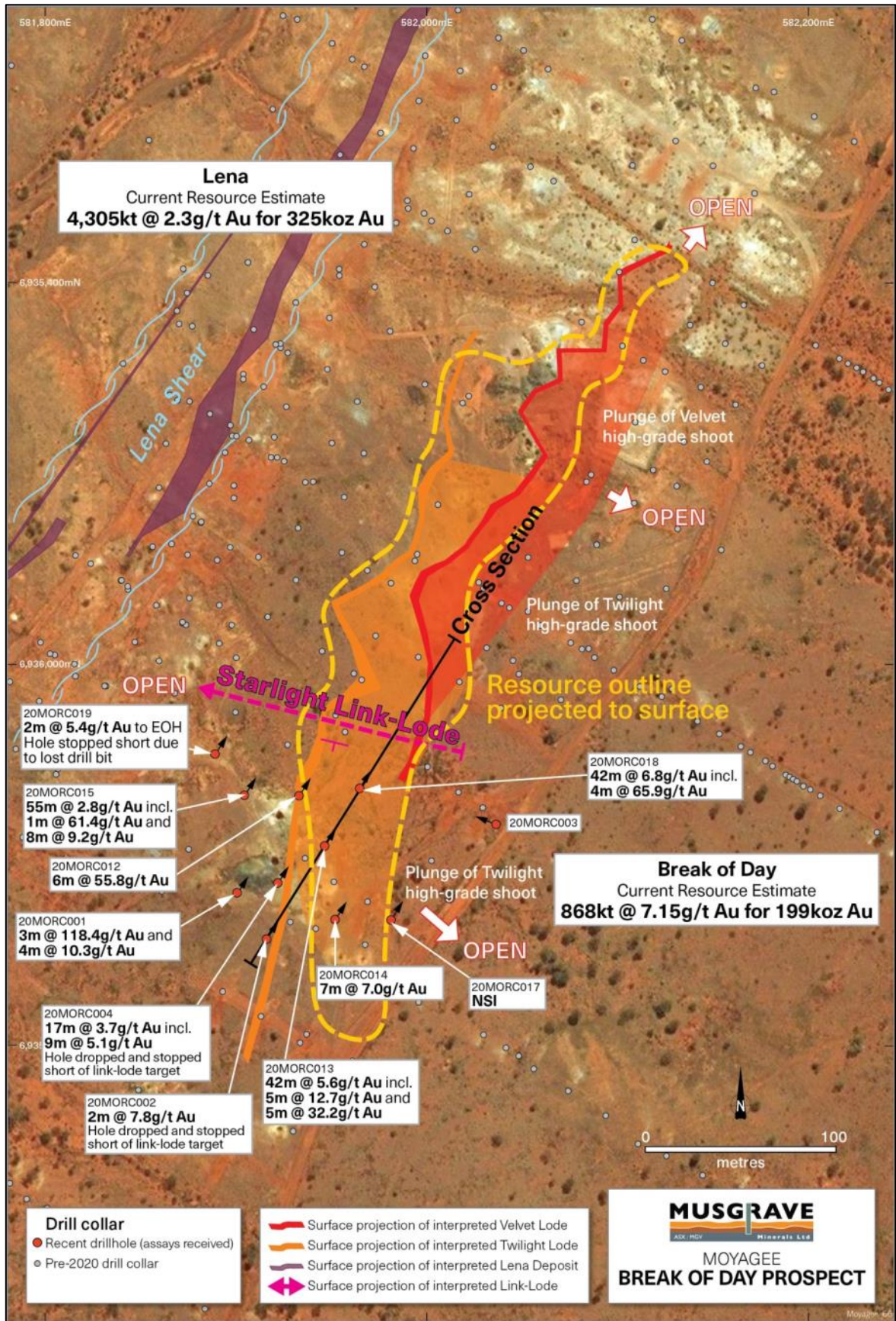
Figure 2: Plan showing Starlight link-lode position at Break of Day and Starlight drill collars and assay results
